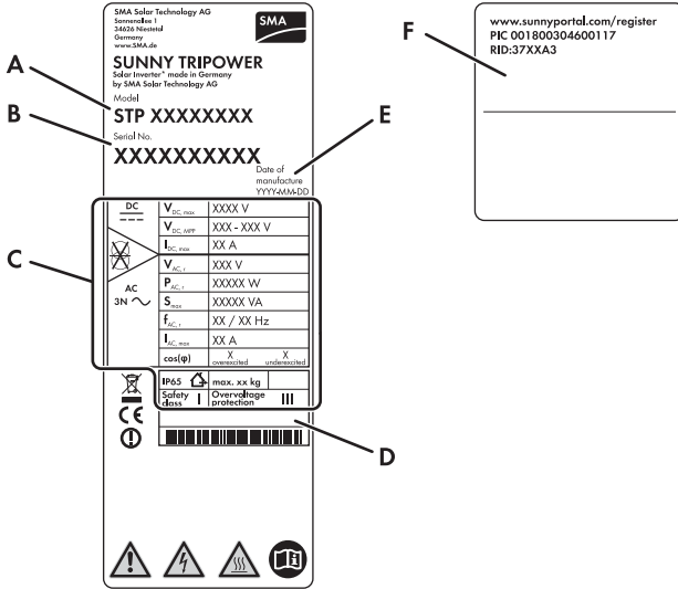
Figure 4: Design of the type label and the additional sticker
