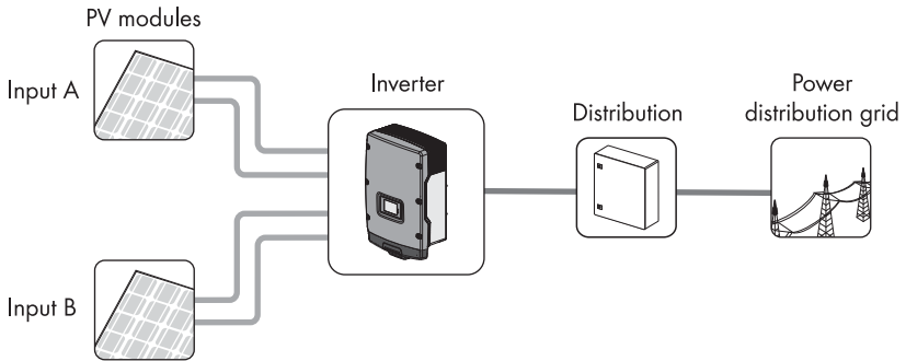
Figure 1: Design of a PV plant with Sunny Tripower
