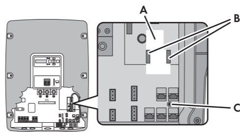
Figure 2: Installation location and connection of the interface
