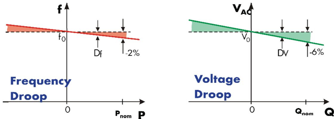
Figure 8.5: Self-sync - droop
