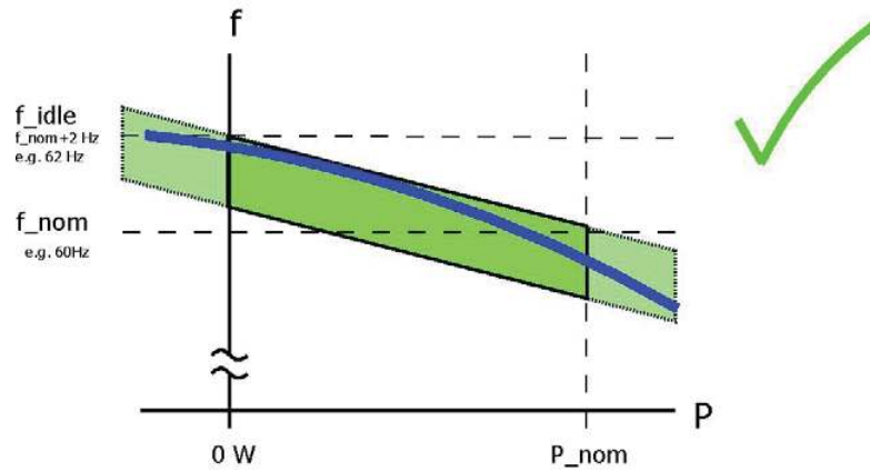
Figure 8.2: Generator behavior: frequency - continuous - suitable
