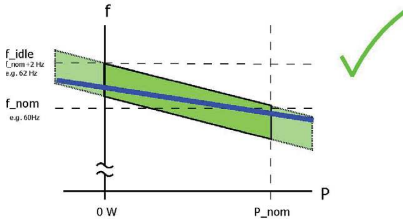
Figure 8.1: Generator behavior: frequency - linear - suitable
