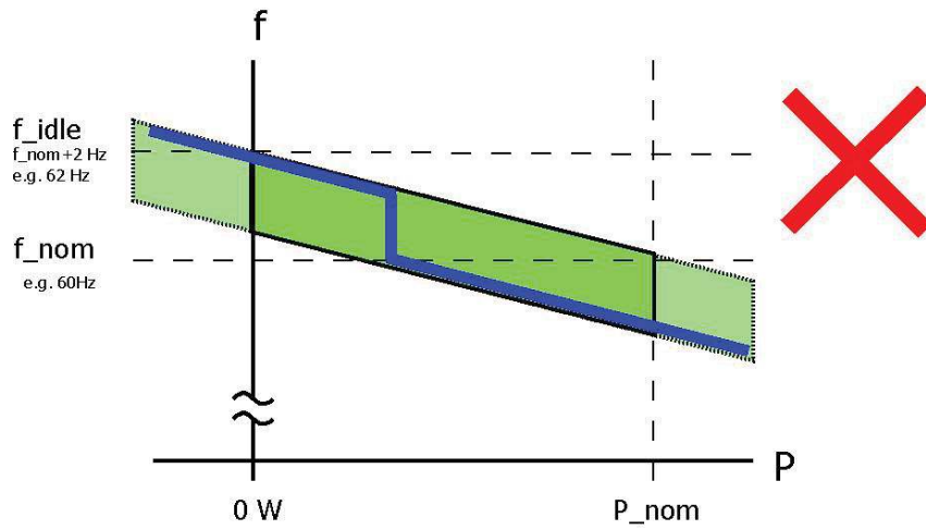
Figure 8.3: Generator behavior: frequency - discontinuous - not suitable
