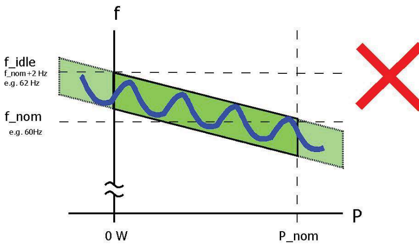
Figure 8.4: Generator behavior: discontinuous frequency - not suitable
