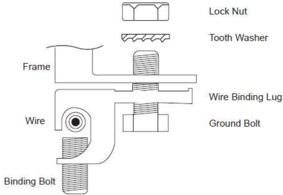
Figure 7: Installation Methods
