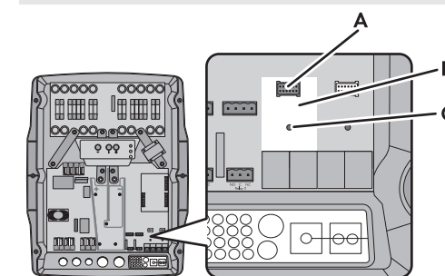
Figure 2: Installation position and connection of the SI-COMSMA.BG1
